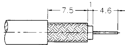
RECOMMENDED CABLE STRIPPING DIM'S (STEP 1) (建議剝線尺寸)
